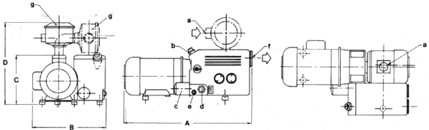
a - Inlet (Pipe Thread) b - Oil Fill Plug c - Oil Filter d - Oil Sight Glass e - Oil Drain Plug f - Exhaust g - Inlet Dust Filter
